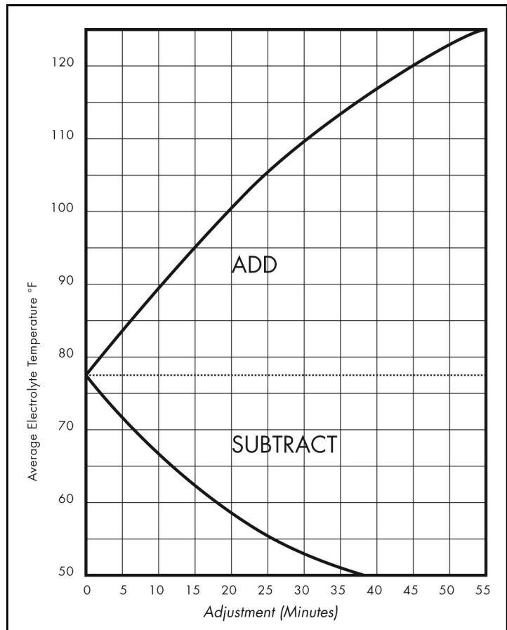
Temperature Correction for Capacity Testing
