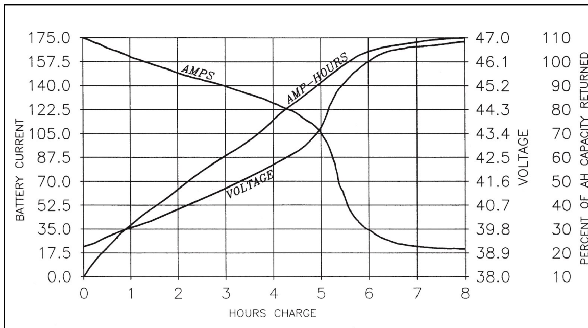
Typical Recharging Characteristics. Typical charge return to an 18-cell battery discharged at 80%, using a HAWKER® LIFE GUARD® charger.
