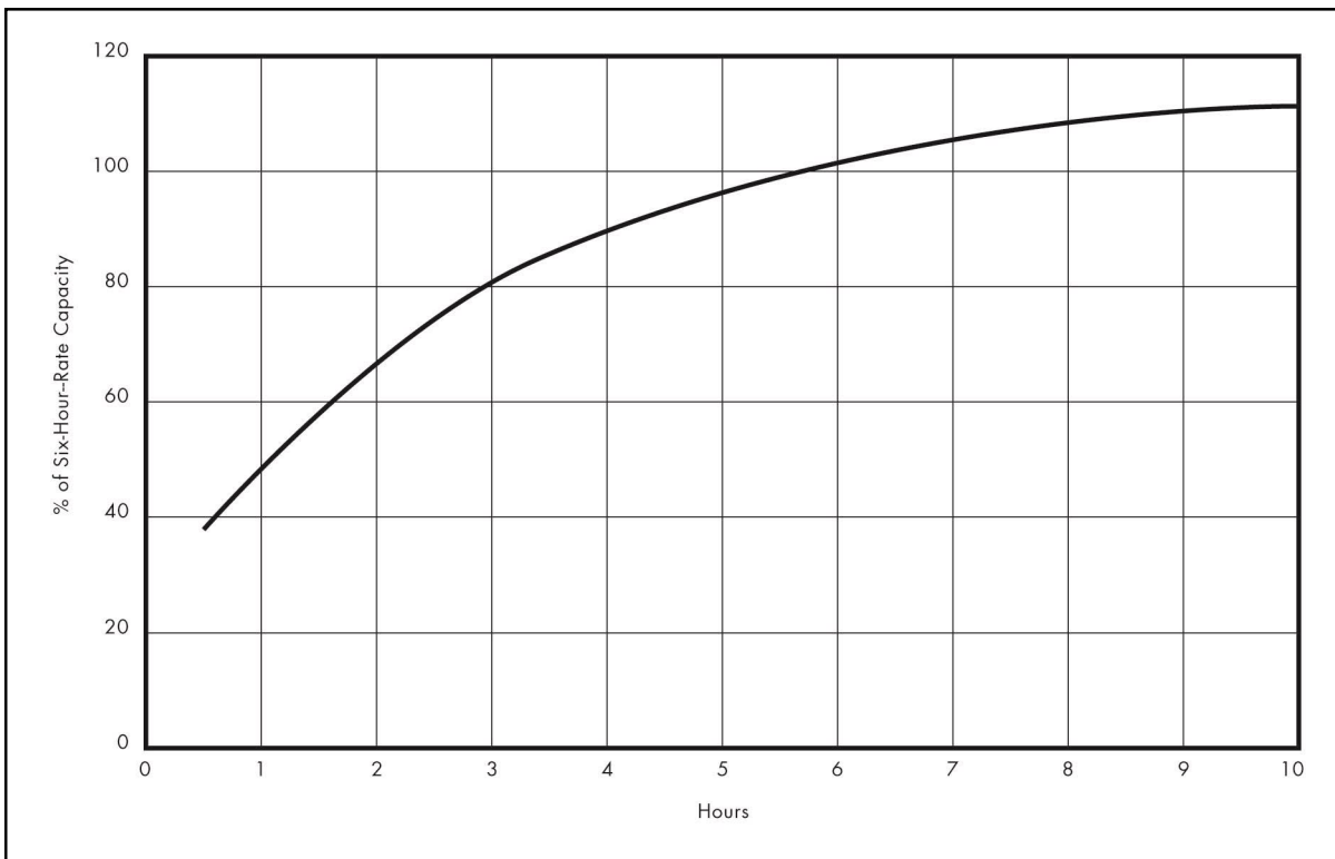
Percentage of Available Capacity vs. Rate of Discharge
