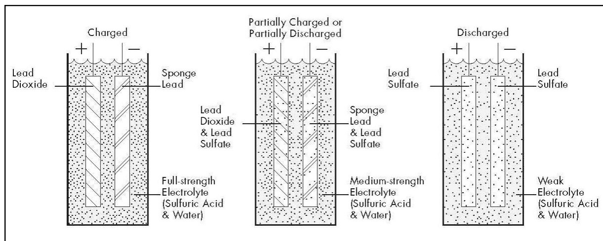
The Charge / Discharge Process
