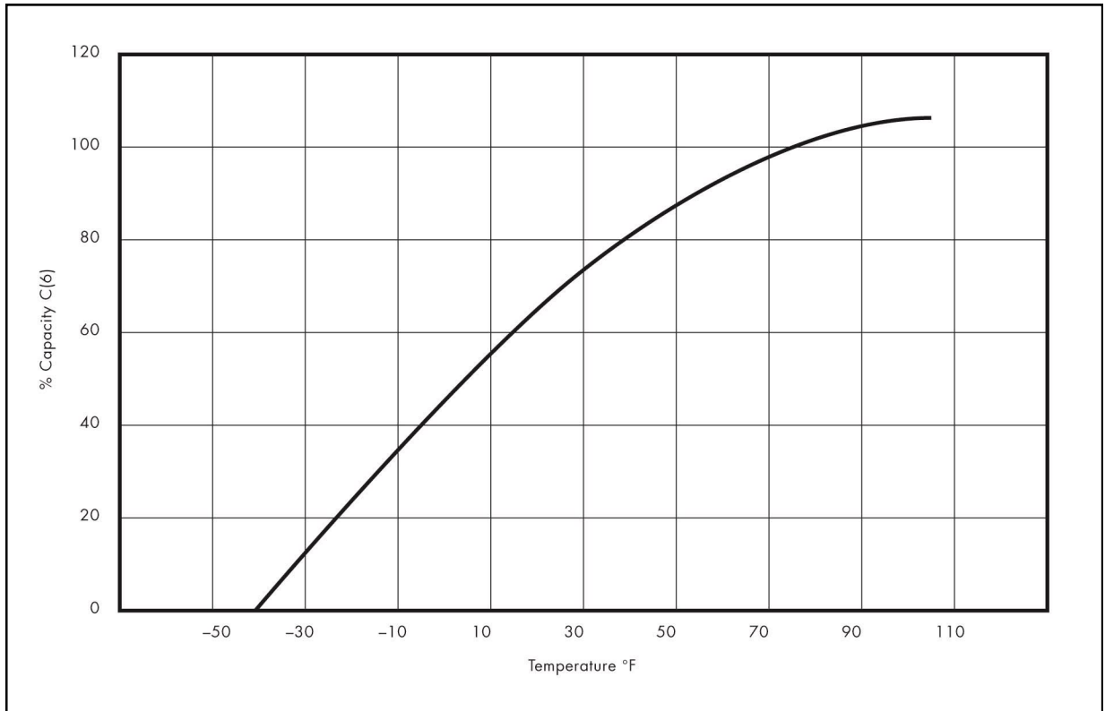
Available Capacity vs. Temperature
